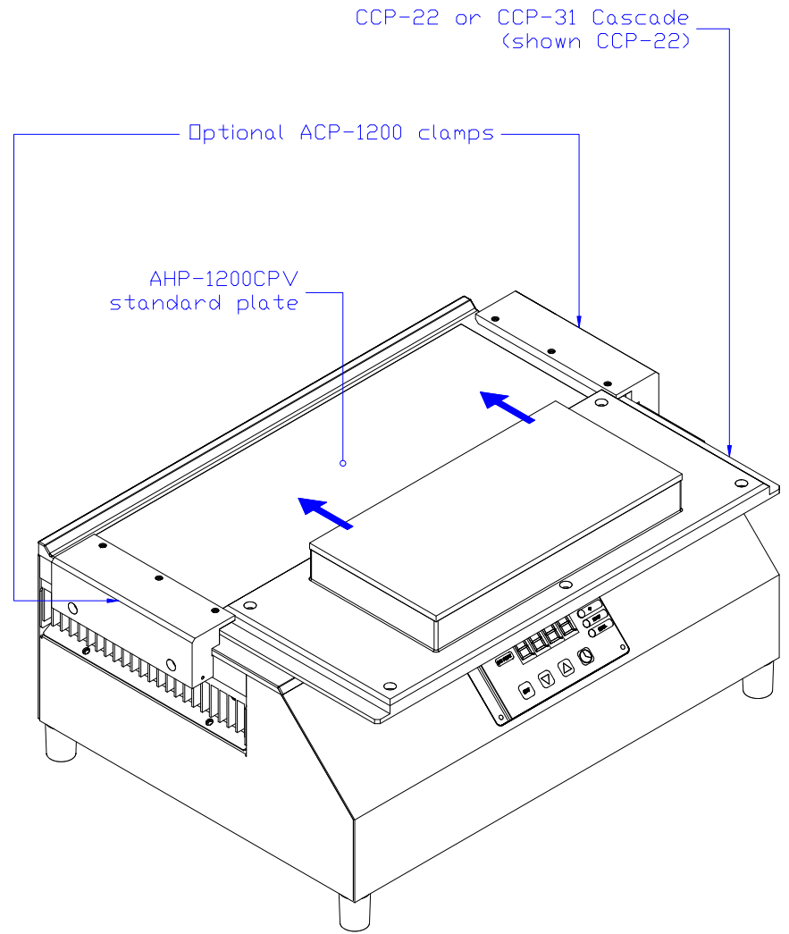
Installation of CCP-22 or CCP-31 via optional ACP-1200 clamps on AHP-1200CPV built with standard plate
