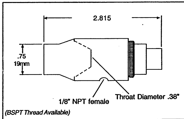
High-Thrust Jet Model 38044
