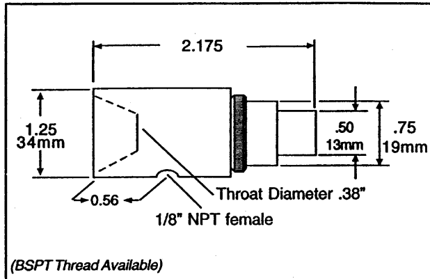
High-Thrust Jet Model 38038
