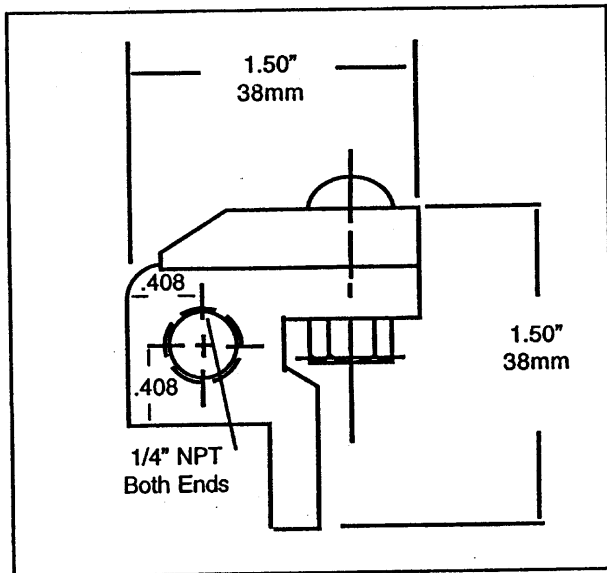
End View Aluminum Air Curtain
