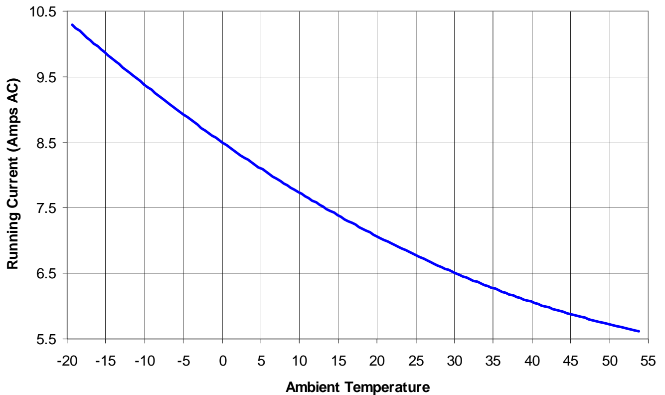
AHP-2252 Running Current, 244.5 VAC Avg
