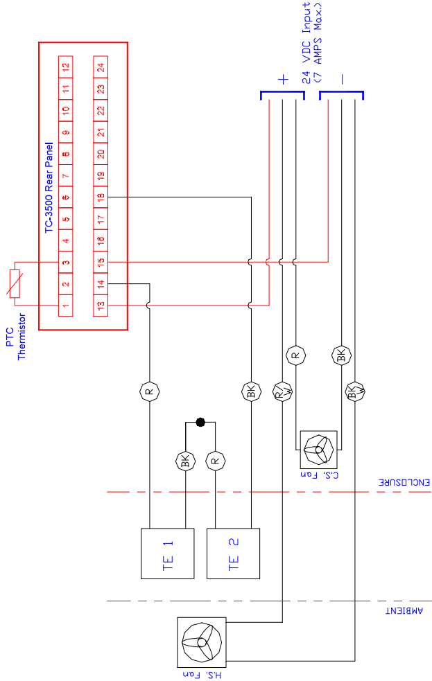
24 VDC, Heat/Cool with TC-3500 (shown in RED)
