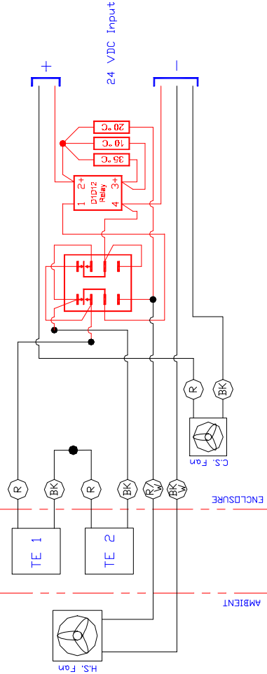
24 VDC, Heat/Cool with TC-7F (shown in RED)
