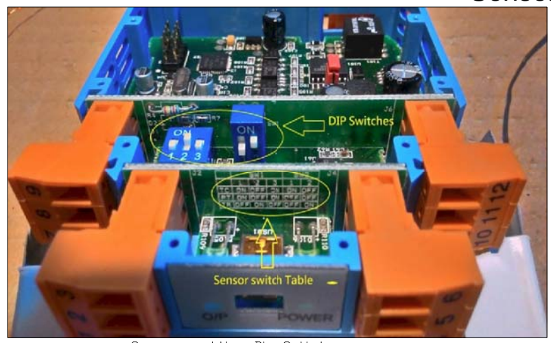
Sensor setting Dip-Switches
